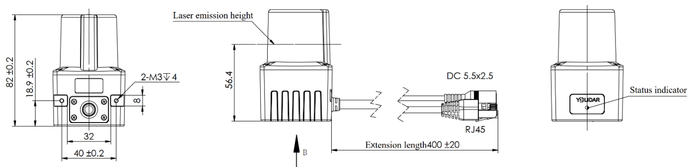
FIG 2 YDLIDAR TIA-H MECHANICAL DIMENSION (UNIT:MM)
